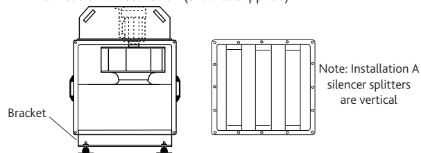
Figure 2. End view of non-recommended horizontally mounted unit installation (bracket by others).
